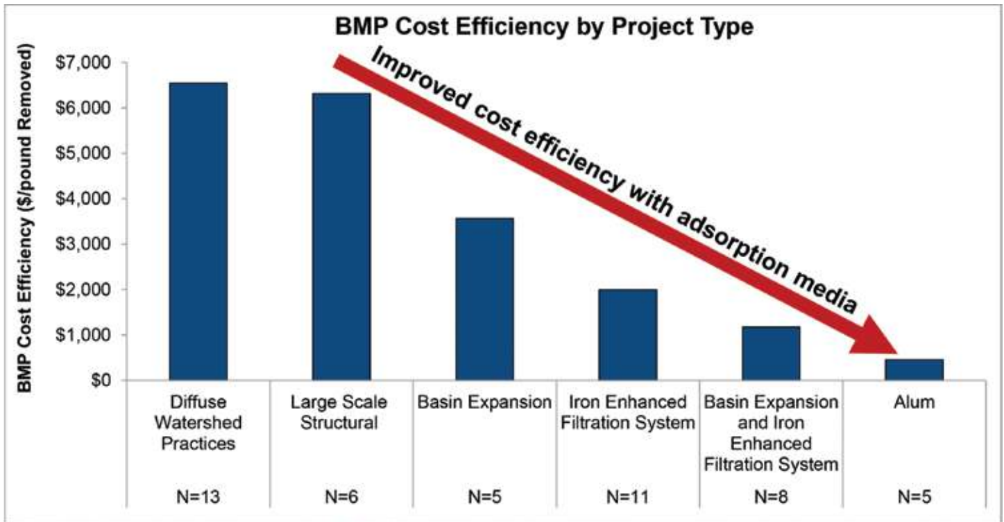
Figure 4. Project cost and phosphorus removal efficiency for watershed and in-lake Best Management Practices.
