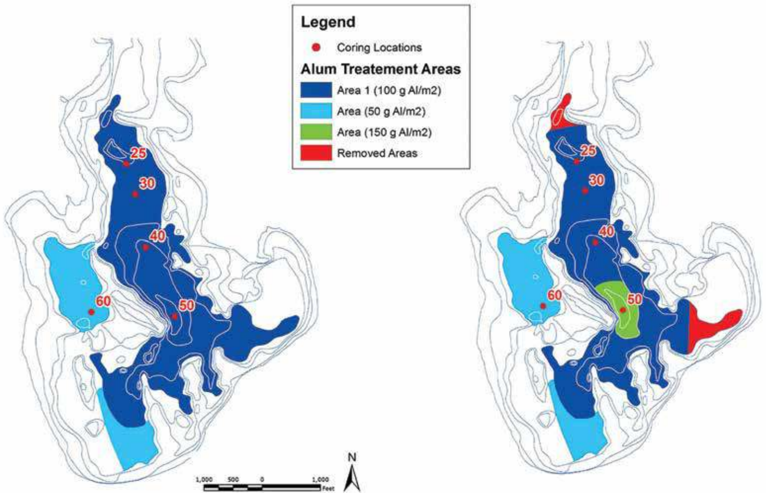
Figure 7. Alum application areas and rates used in the initial half dose applied in spring of 2014 and the adjusted half dose applied in spring of 2016.
